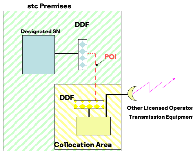
figure 3.1: Collocated Interconnection
